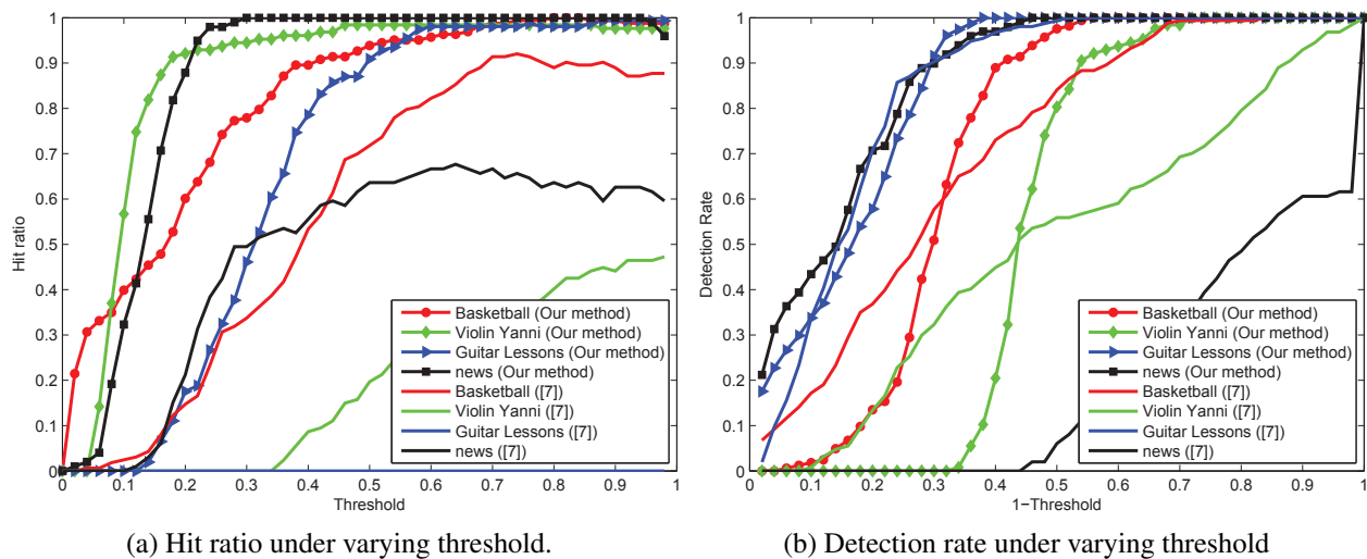
Figure 3.7: Quantitative results of temporal localization performance.
