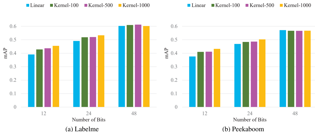
Figure 4.4: Evaluation of the kernel space extension. The subspace dimension is set to 4 for all the variants of SRH. “Linear” is the default SRH. “Kernel-100”, “Kernel-500”, and “Kernel-1000” represent the kernelized SRH with 100, 500 and 1000 anchors respectively. The kernel version of SRH generally performs better than the default SRH with linear subspace rankings.
